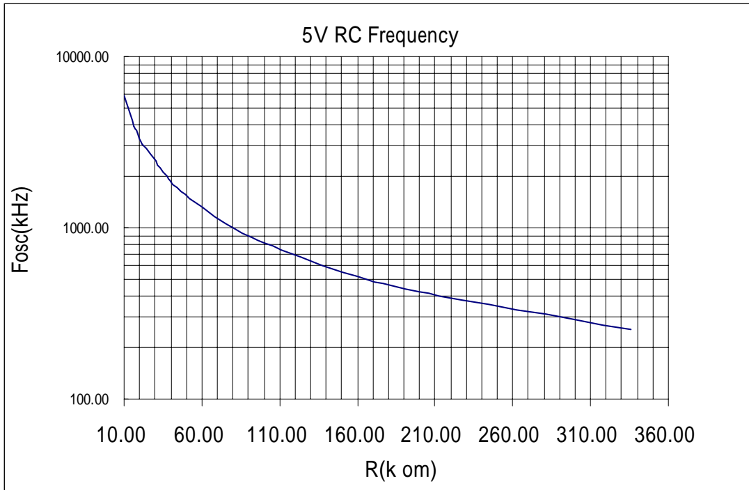
Typical RC oscillator Resistor vs. Frequency: ( V_{DD} = 5V , for reference only)
